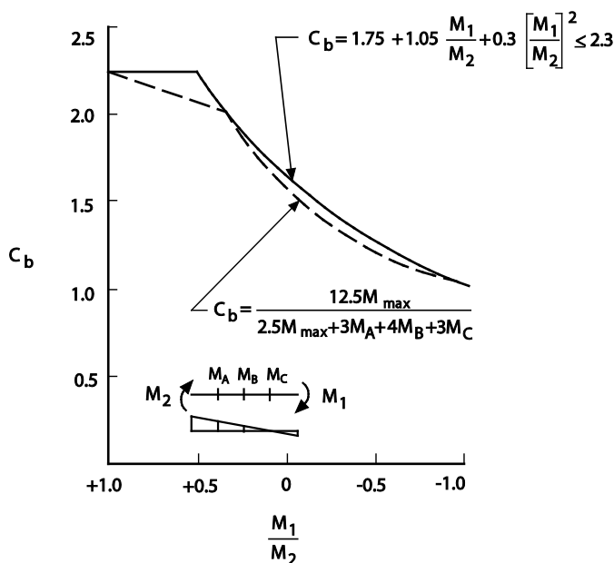
Figure C-2.3.1.2-1 C_b for Straight Line Moment Diagram
