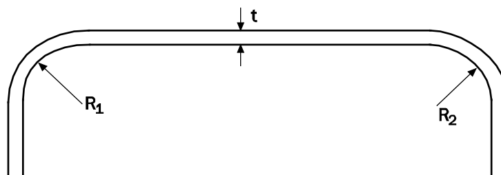
Figure C-B4.1-1 Corner Radius
