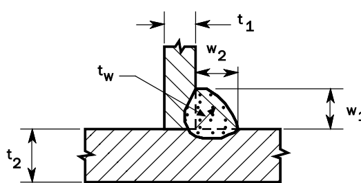
Figure J2.6-2 Fillet Welds – T-Joint
