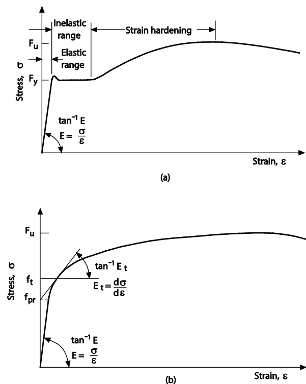
Figure C-A3.3.1-1 Stress-Strain Curves of Carbon Steel Sheet or Strip
