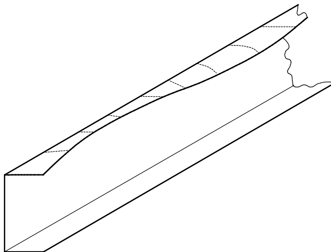
Figure C-1.2-1 Local Buckling of Unstiffened Compression Flange
