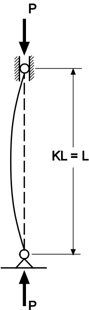
Figure C-2.3.1.1-1 Overall Column Buckling
