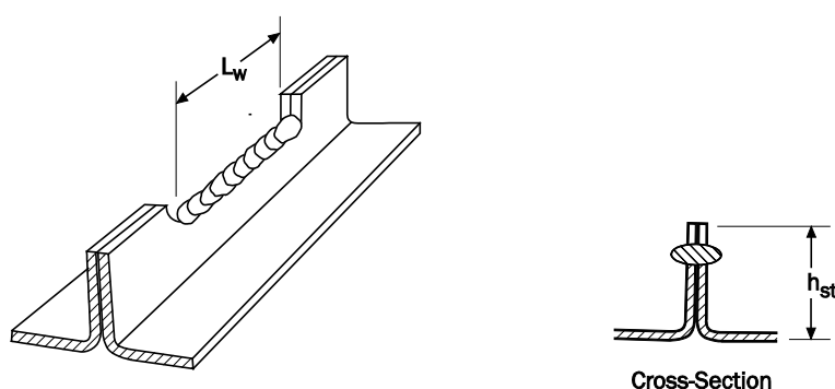
Figure J2.4.1-1 Top Arc Seam Sidelap Weld
