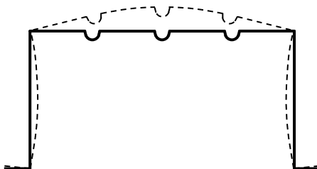
Figure C-E4-2 Distortional Buckling of Element With Intermediate Stiffeners
