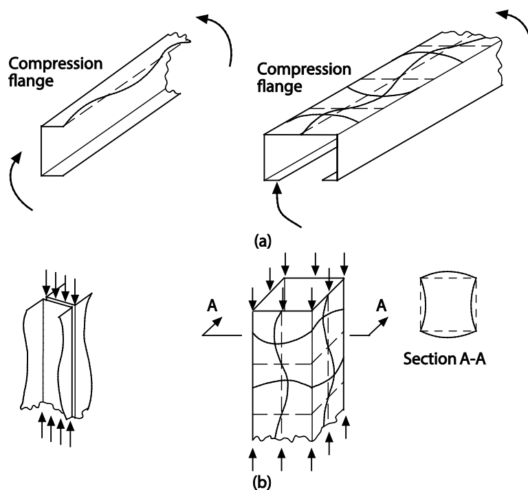
Figure C-1-1 Local Buckling of Compression Elements: (a) Beams, (b) Columns
