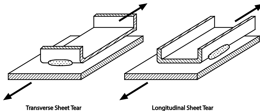
Figure C-J2.7-1 Flare Groove Weld Failure Modes
