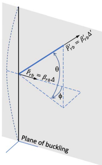
Figure C-C2.3.1-1, Non-Perpendicular Brace
